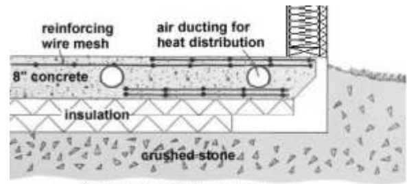
Slab Section View
