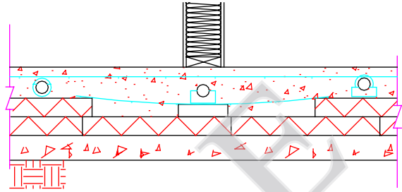
SLAB SECTION - BEARING WALL
