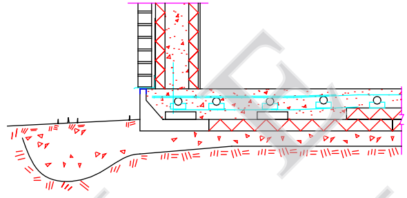
ICF WALL with BRICK FINISH
