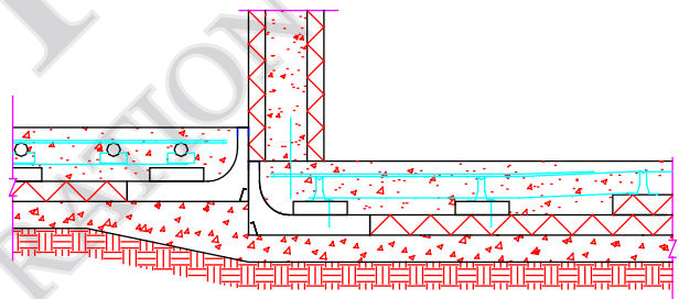
STEP BETWEEN HEATED and UNHEATED SLABS
