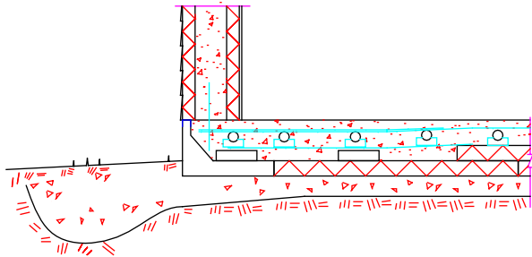
ICF WALL with SIDING FINISH
