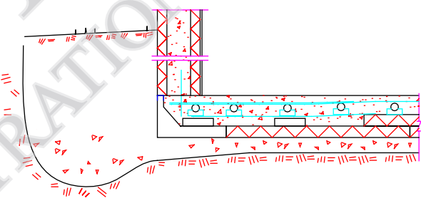
PARTIALLY BURIED ICF WALL
