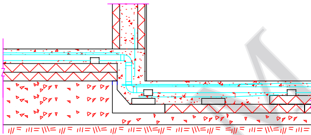
STEPPED SLAB SECTION
