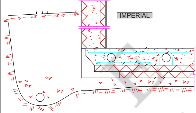
PARTIALLY BURIED ICF WALL
