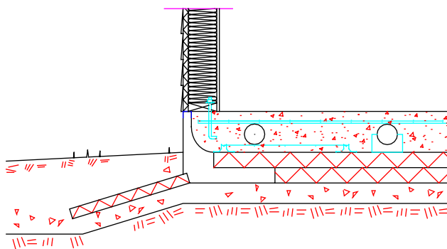
STICK FRAME WALL with SIDING FINISH - SKIRTED SLAB
