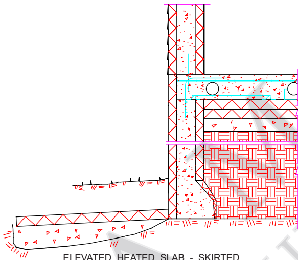
ELEVATED HEATED SLAB - SKIRTED
