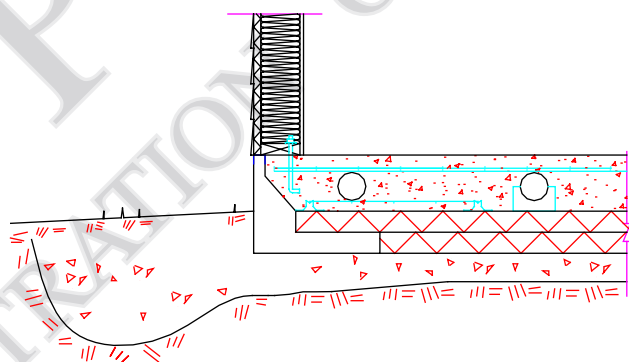
STICK FRAME WALL with SIDING FINISH
