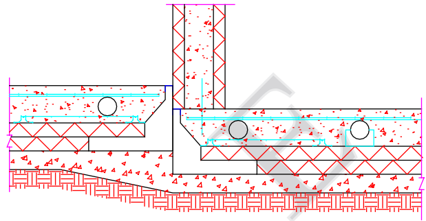
STEP BETWEEN HEATED SLABS
