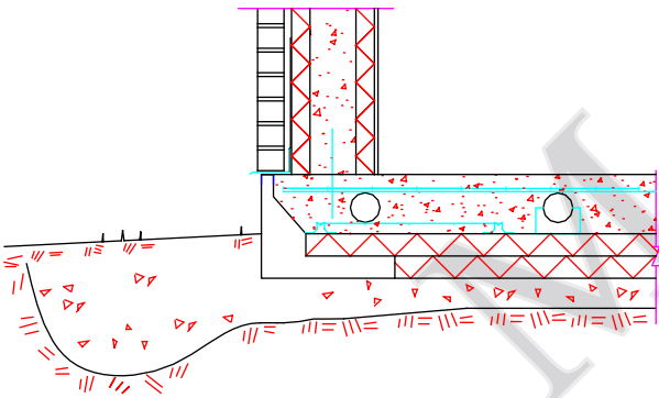
ICF WALL with BRICK FINISH
