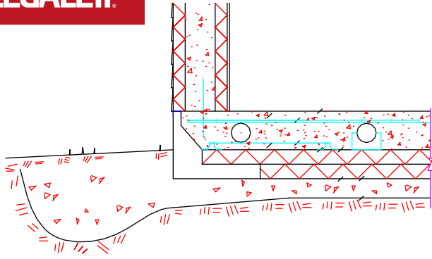
ICF WALL with SIDING FINISH
