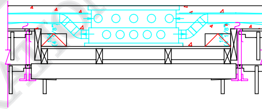
HAMBRO / LEGALETT FURNACE BOX
