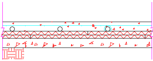
4 INCH SLAB SECTION - 2 INCH PIPE
