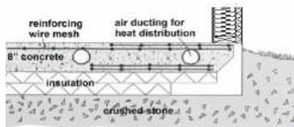
Slab Section View
