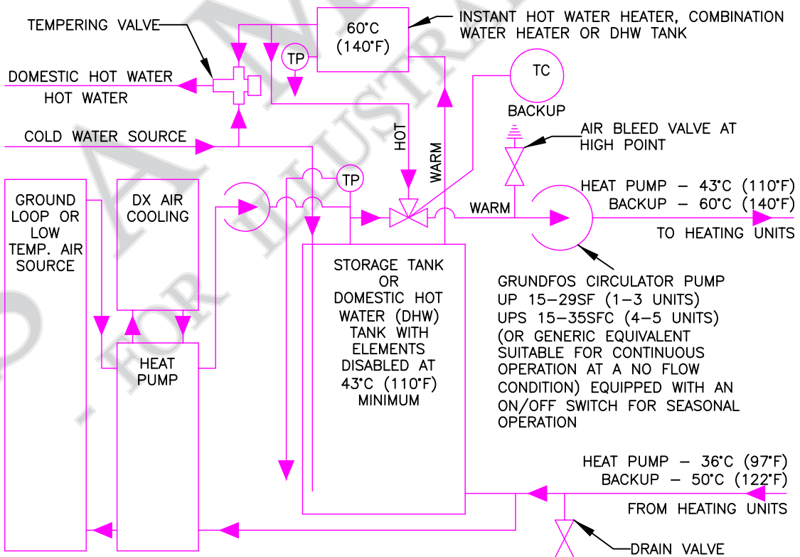
TYPICAL OPEN LOOP HEAT PUMP HOT WATER SUPPLY – BY OTHERS
