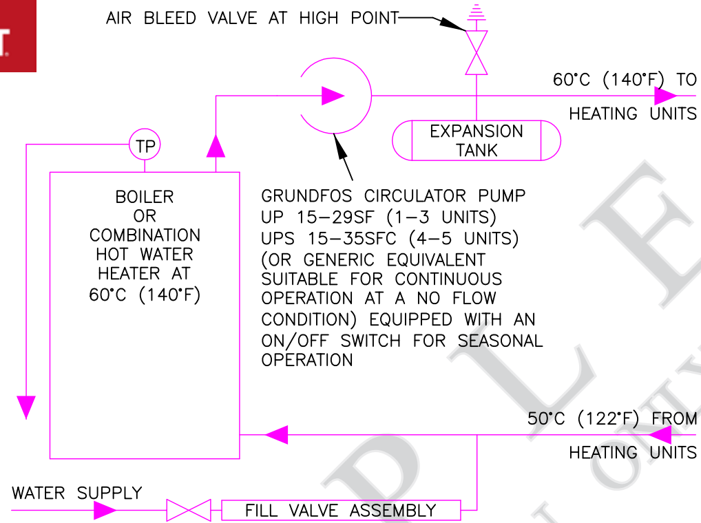
TYPICAL CLOSED LOOP HOT WATER SUPPLY – BY OTHERS
