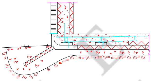
ICF WALL with BRICK FINISH HEATED BUILDING on 5" UNHEATED SKIRTED SLAB
