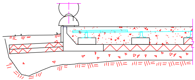
LOG WALL with BASE LOG HEATED BUILDING on 5" UNHEATED SKIRTED SLAB
