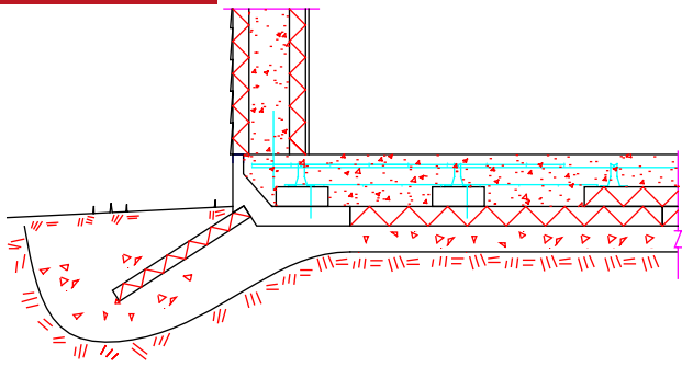
ICF WALL with SIDING FINISH HEATED BUILDING on 5" UNHEATED SKIRTED SLAB
