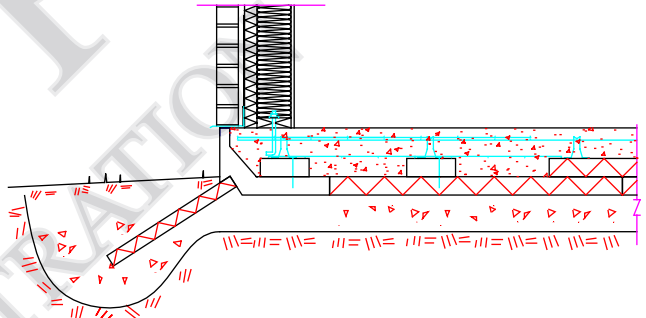
STICK FRAMED WALL with BRICK FINISH HEATED BUILDING on 5" UNHEATED SKIRTED SLAB
