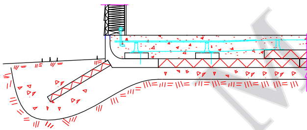
STICK FRAMED WALL with SIDING FINISH HEATED BUILDING on 5" UNHEATED SKIRTED SLAB
