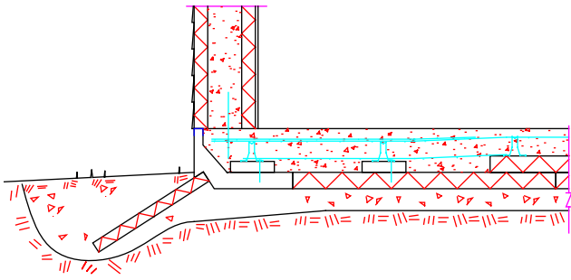
ICF WALL with SIDING FINISH UNHEATED BUILDING on 5" UNHEATED SKIRTED SLAB
