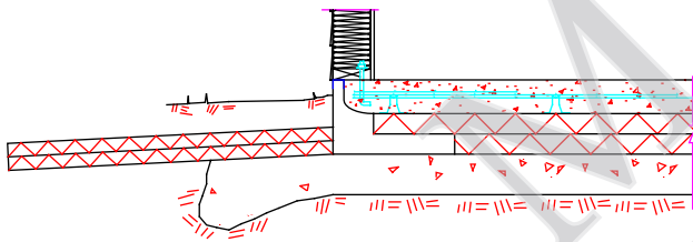
STICK FRAMED WALL with SIDING FINISH UNHEATED BUILDING on 5" UNHEATED SKIRTED SLAB
