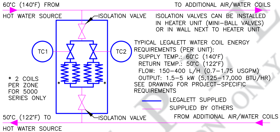
TYPICAL LEGALETT WATER COIL INSTALLATION
