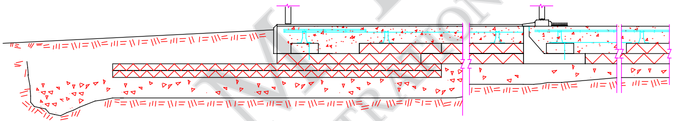
TYPICAL UNHEATED PORCH - POST LOAD
