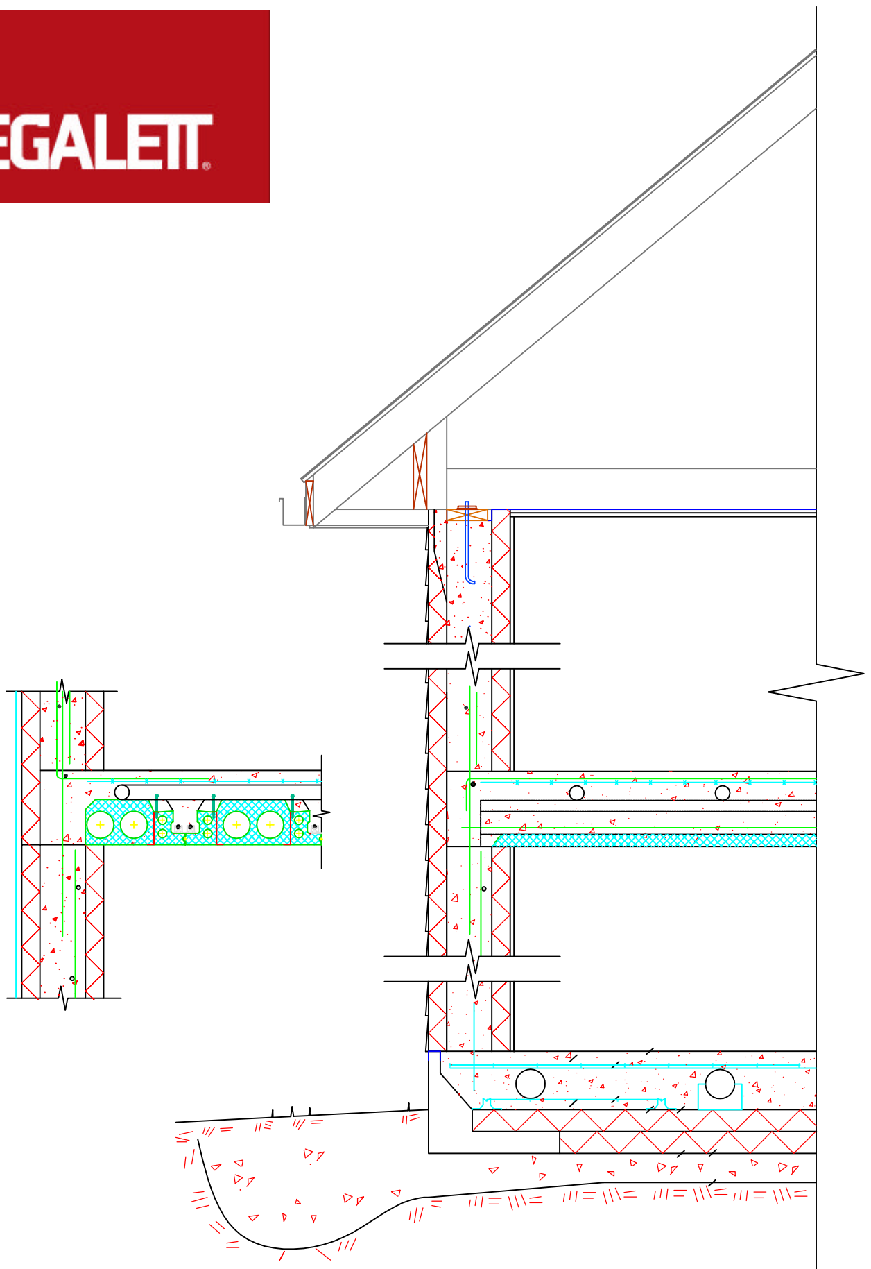
TYPICAL SECTION—CAST—IN—PLACE INSULATED SUSPENDED FLOOR (INSUL—DECK, LITE—DECK, ETC.)
