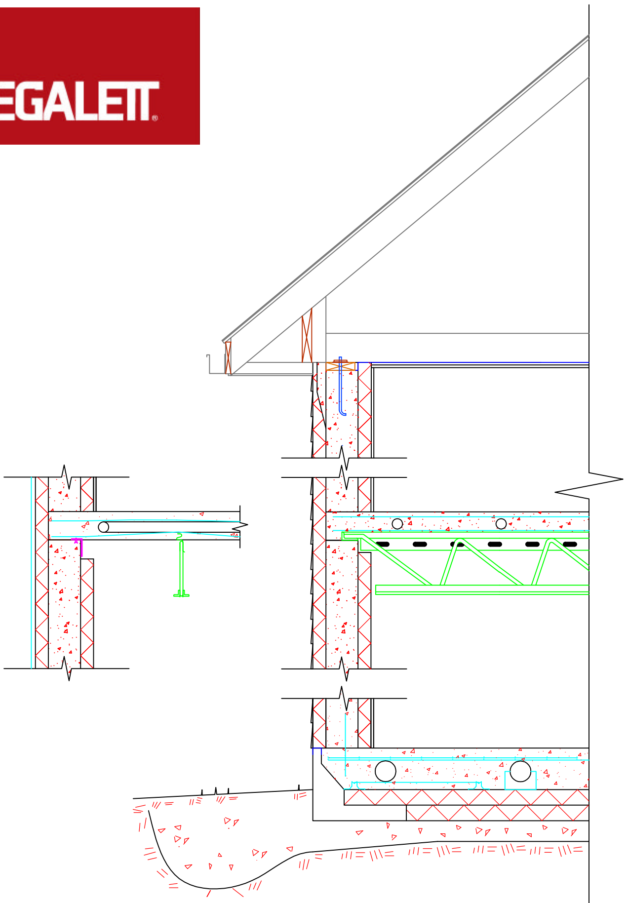
TYPICAL SECTION—CAST—IN—PLACE OPEN WEB COMPOSITE SUSPENDED FLOOR (HAMBRO, ETC.)
