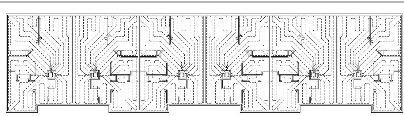
Heater and Pipe Layout
