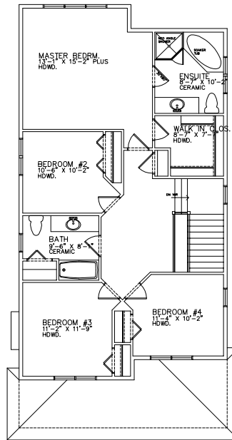
SECOND FLOOR PLAN 1156 SQ.FT.
