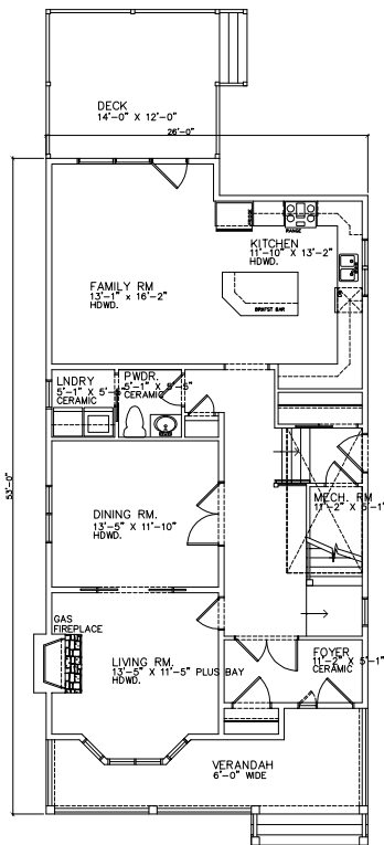
GROUND FLOOR PLAN 1183 SQ.FT.
