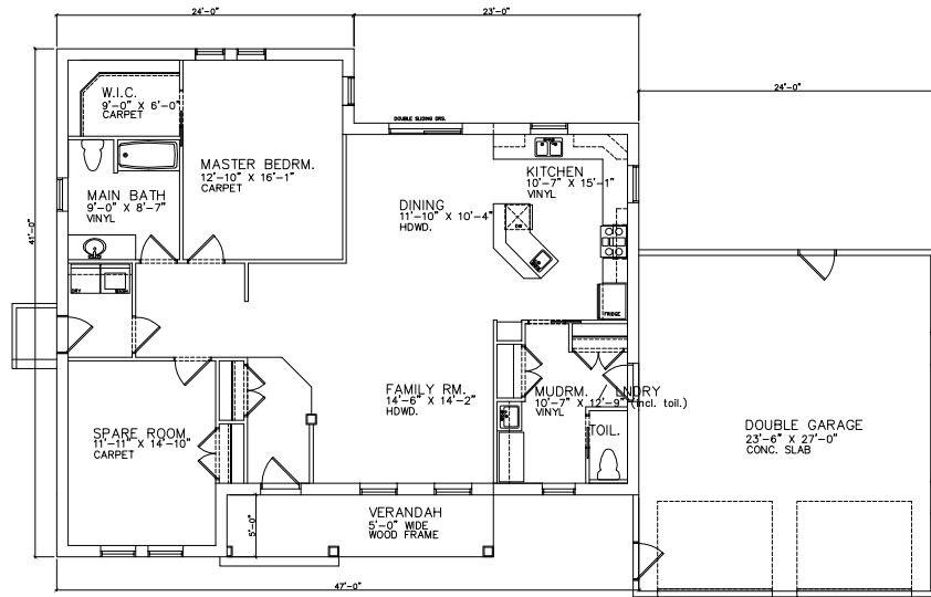
GROUND FLOOR PLAN 1622 SQ.FT.
